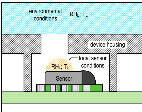
Figure 1: The sensor measures the local conditions at the sensing element ( RH_L; T_L ). In order to achieve good measurements this local conditions need to correspond to the conditions of the environment under test (i.e. RH_E; T_E ).
