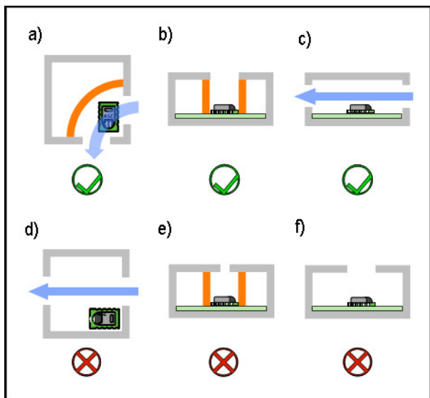
Figure 7: Schematic view of different design-ins. a) This is the preferred design if ever possible. The small dead volume, sufficient aperture size and the air flow allow a fast humidity response time. b) The walls (orange) reduce the dead volume which will lead in combination with the large aperture to fairly good response times. c) The defined airflow goes directly over the sensor and therefore the local conditions at the sensor equilibrate quickly with the environmental conditions. If there is no defined flow this design is not recommended as the dead volume is too big. d-f) This designs will have slow humidity response times due to the following reasons: d) The airflow misses the sensor and the dead volume is large. e) The aperture size is too small in respect to the dead volume. f) The dead volume is large.
