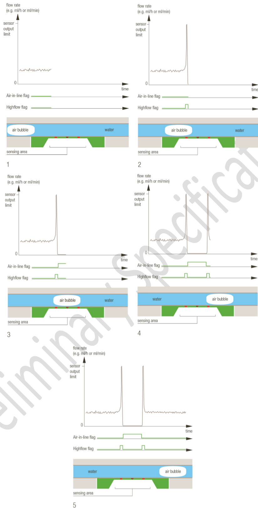
Figure 3: Detection of air-in-line events with the LD20-0600L. The graphs illustrate the air-in-line and high-flow flags while a bubble is passing through the sensor from left to right.
