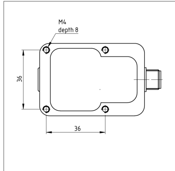
Figure 2: Rear side with drill holes for mounting SONOFLOW CO.55/xxxSD V2.0
