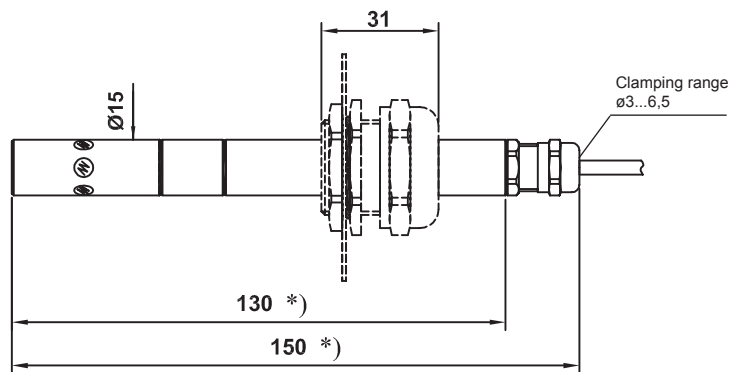
VC series
